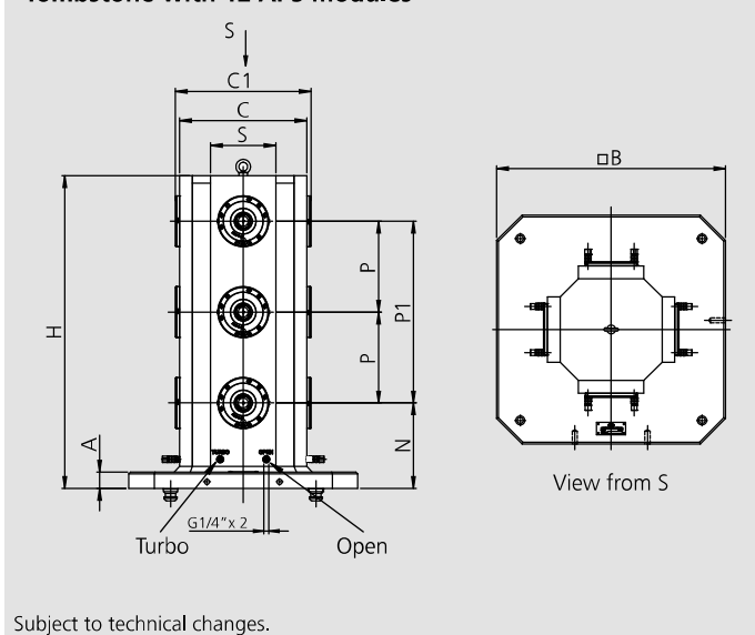
Tombstone with 12 APS modules
