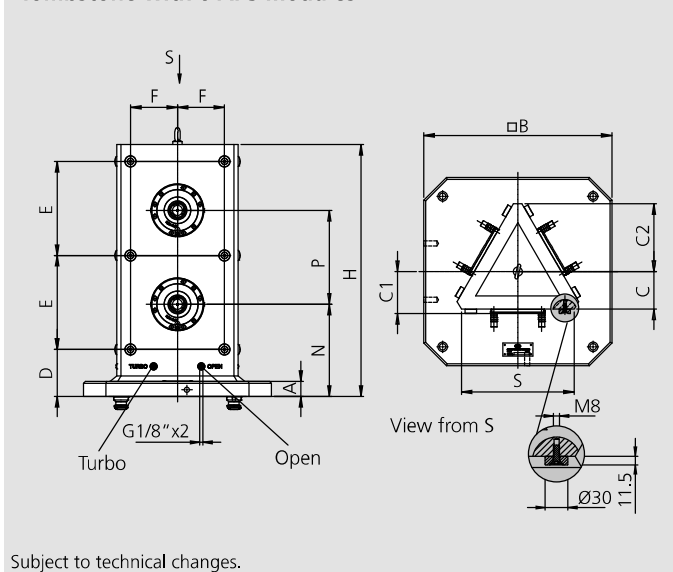
Tombstone with 6 APS modules
