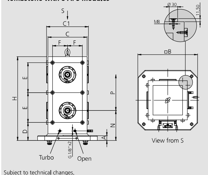
Tombstone with 8 APS modules
