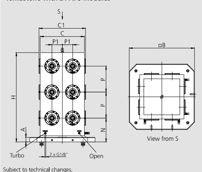
Tombstone with 24 APS modules
