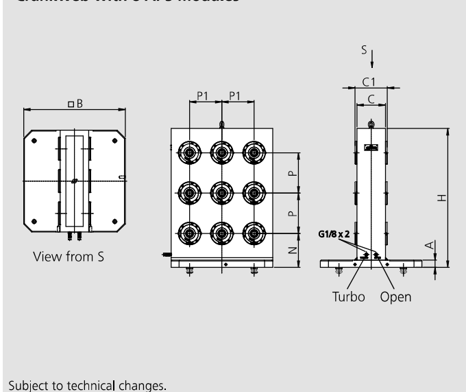
Crankweb with 8 APS modules
