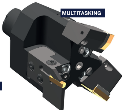
SPECIAL BORING BAR
