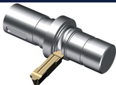
RADIUSFORM CUTTING
